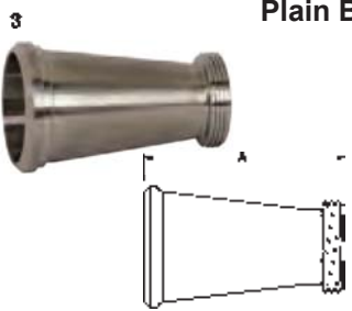
Threaded Bevel Seat x Plain Bevel Seat with Hex Nut Concentric Reducers - B31TP
