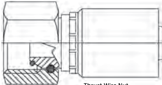
Thrust-Wire Nut
