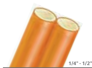
BR7 SAE 100R7 (Twin-Line, Non-Conductive) Medium-pressure, twin-line thermoplastic hose with a non-perforated cover.
